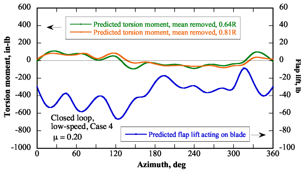
Fig. 6j. Predicted effect of flap on blade, closed loop Case 4.
