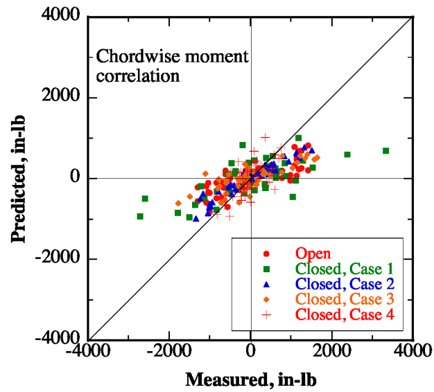
Fig. 7c. Chordwise moment correlation.
