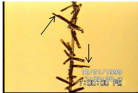
100 \mu\text{m} (glass thread is 50 \mu\text{m} ); steps indicated by arrows
