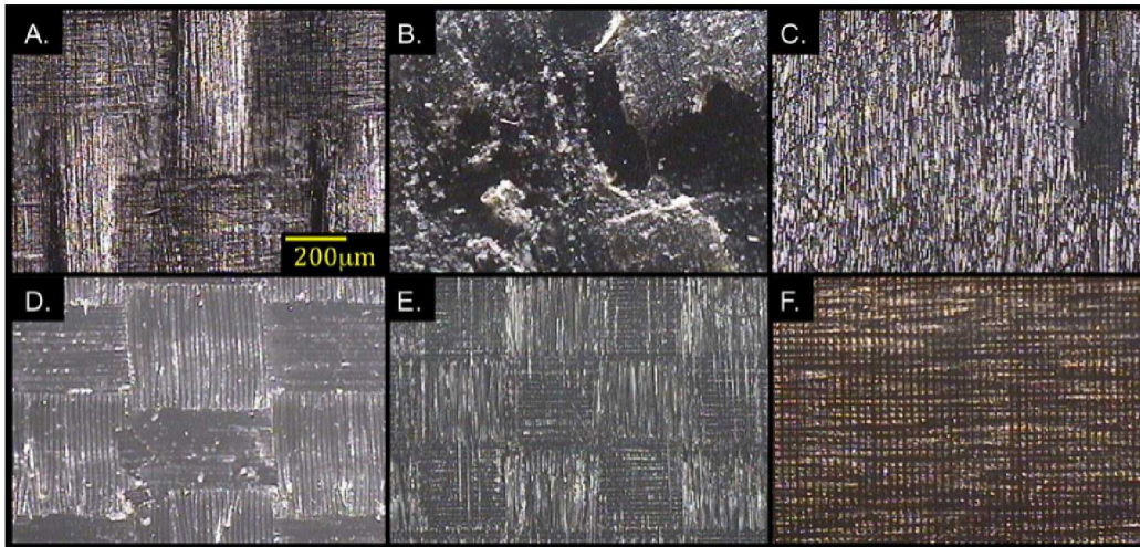
Figure 3. CFRP surface (A.) as is, (B.) grit blasted, (C.) manually abraded, (D.) treated with peel ply, (E.) laser etched with pattern A from Figure 1, and (F.) laser etched with pattern B from Figure 1.
