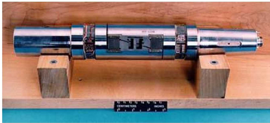
Figure 1 Typical Six Degree of Freedom Internal Wind Tunnel Force Balance
