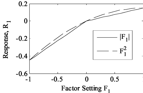
Figure 7 Asymmetric Slope Modeling Comparison
