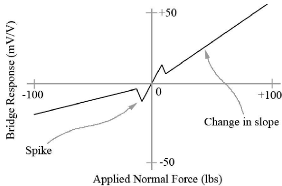
Figure 2 Non- Monolithic Force Balance Response due to Applied Force
