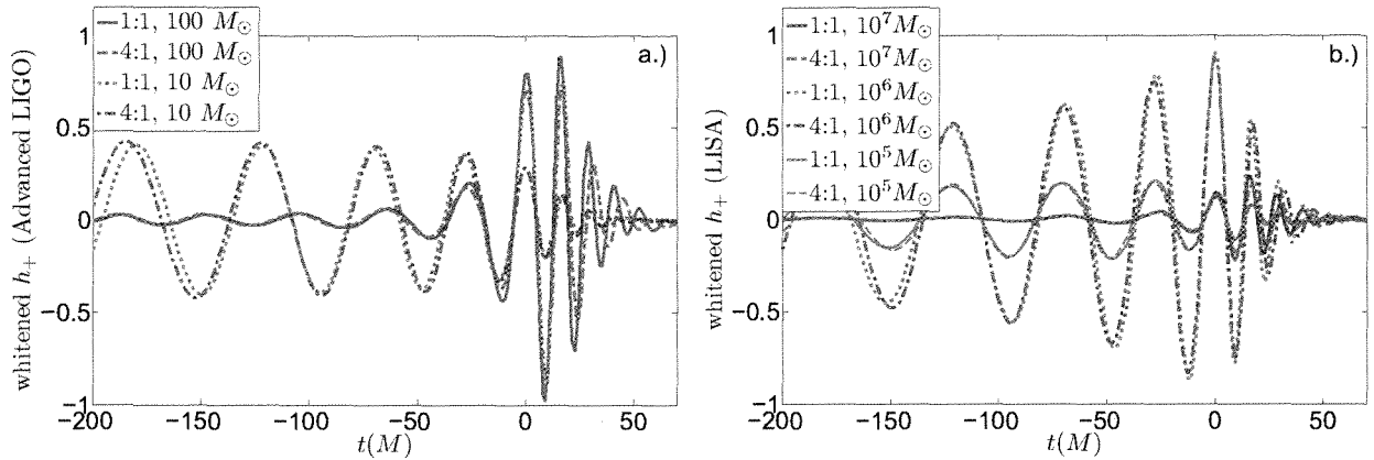
FIG. 11: Examples of “whitened” waveforms [32] that we use to form a basis for calculating the match. Examples for Advanced LIGO are shown in the left panel, and examples for LISA are shown in the right panel. The ordinate values are arbitrarily scaled.
