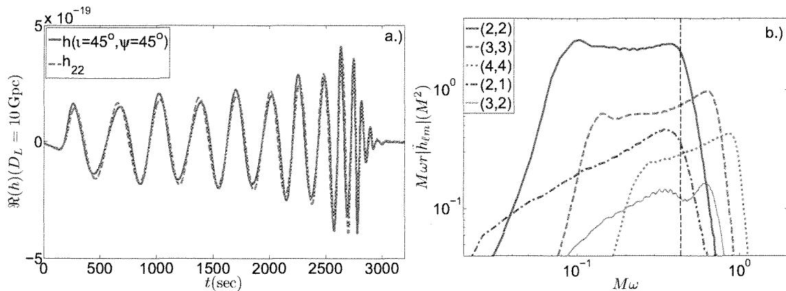
FIG. 8: In the left panel, we show a time series representation of a 6:1 mass-ratio 10^6 M_\odot black-hole binary at a distance of 10 Gpc, using the waveforms from our numerical simulation. This is a typical example of the (2, \pm 2) modes constituting the vast majority of the overall power content of the waveform. This is further demonstrated in the Fourier-series representation (right panel), where the (2, \pm 2) modes dominate until well into the ringdown, the onset of which is approximately indicated by the dashed vertical line.
