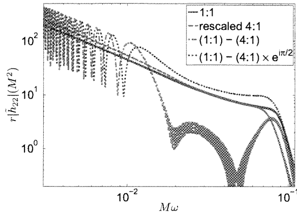
FIG. 7: The Fourier amplitude of the waveform difference in Fig. 6, both with the phase shift shown there, as well as shifted by \pi/2 to illustrate the dependence of the power at high frequencies on the phase alignment.
