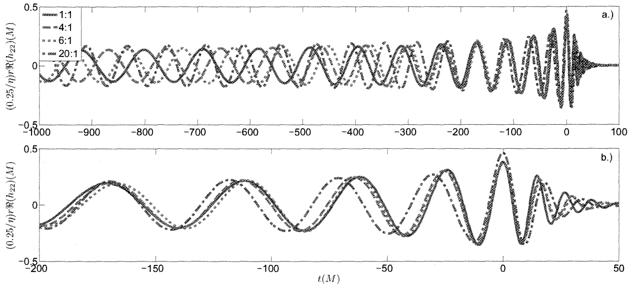
FIG. 2: In the top panel, we show quadrupole waveforms generated by using the model presented in [15] for mass ratios of 1:1, 4:1, 6:1, and 20:1. When the waveforms are aligned in time based on their peak amplitudes, and aligned in phase to agree at said time, there is significant overlap of the waveforms for the 1:1, 4:1, and 6:1 cases over the final \sim 5 cycles leading up to merger (shown more clearly in the bottom panel).
