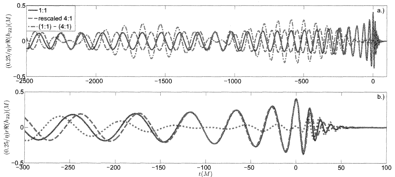
FIG. 6: Differences in 1:1 and rescaled 4:1 mass ratios.
