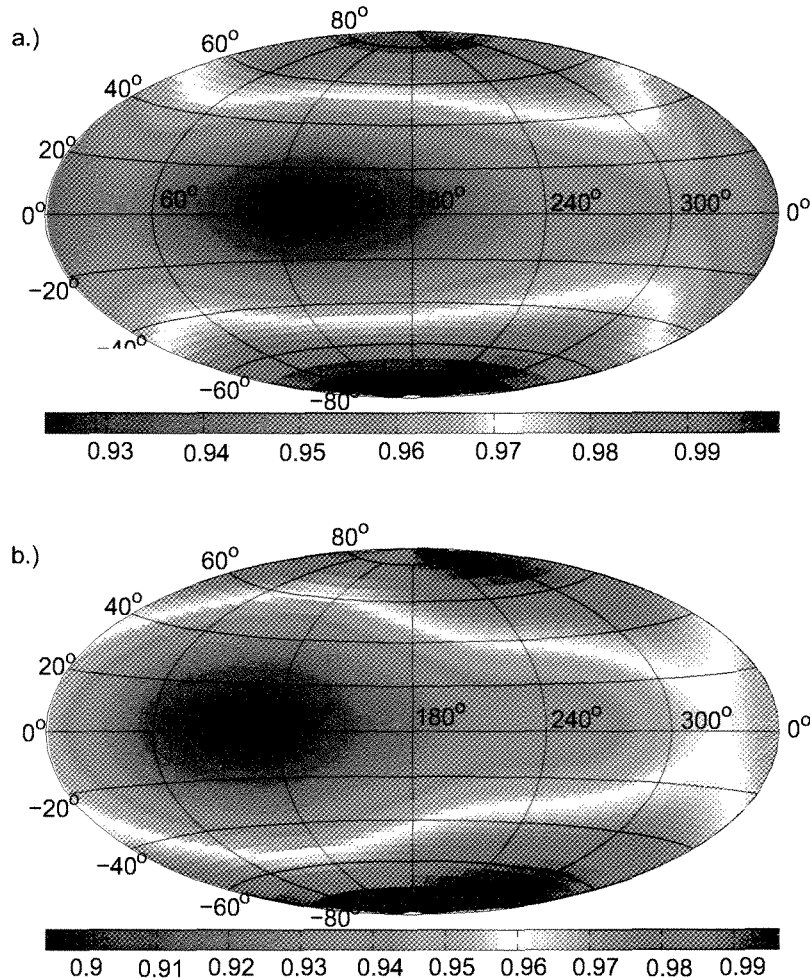
FIG. 10: Sky map of matches between the equal-mass and 4:1 waveforms for Advanced LIGO (a.) and LISA (b.). Throughout the text, \Phi is the azimuthal coordinate and \Theta is the polar coordinate. The specific case shown corresponds to a redshifted mass of M = 100M_\odot for Advanced LIGO, and M = 3 \times 10^6 M_\odot for LISA (the luminosity distance is irrelevant for this calculation), but the result will be qualitatively similar for any mass M \geq 100M_\odot for Advanced LIGO and M \geq 2 \times 10^6 M_\odot for LISA, due to the constancy of the detector response and the similar spectral content of the noise over the band of the signal for those cases, i. e. cases where the “whitening” procedure (see the Appendix) emphasizes the merger. The sky location corresponds to the position on the sky of the equal-mass waveform, with the 4:1 waveform being rotated in the \Phi direction to maximize the match. Therefore, for a fixed \Theta , the maximum in \Phi will correspond to the “best” match, and the minimum to the “minimax” match.
