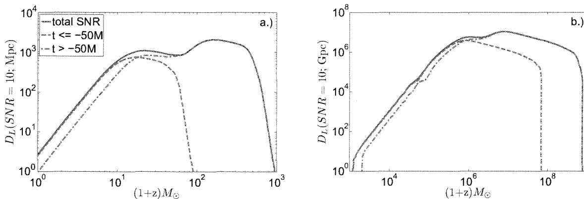
FIG. 9: Luminosity distance where the difference between the 1:1 and rescaled 4:1 mass ratio waveforms is detectable with an SNR of 10 for initial LIGO and LISA, also referred to as the distance horizon. This can be interpreted as being the maximum distance at which we can distinguish these two sources with each interferometer.
