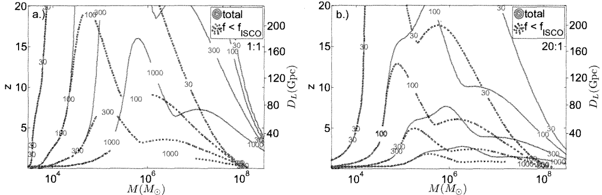
FIG. 5: SNR contours for LISA with q = 1 (a.) and q = 1/20 (b.). The solid lines again correspond to the full waveform SNR, while the dotted lines correspond to the SNR contribution from frequencies lower than the Schwarzschild ISCO frequency. While the observable range of high-SNR mergers is reduced by a factor of several at 20:1 from what was seen in the 1:1 case, sources are still easily detectable to large redshift over a similarly broad mass range.
