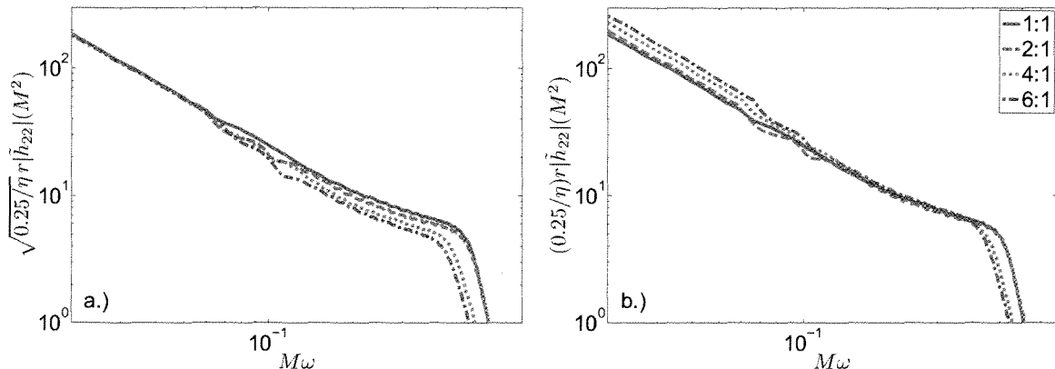
FIG. 3: Scaling of the Fourier amplitude for different mass ratios by \sqrt{\eta} in the left panel (a.), and by \eta in the right panel (b.), which appears to be an excellent approximation.
