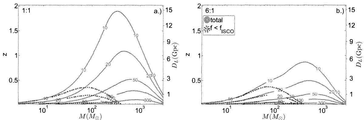
FIG. 4: SNR contours for Advanced LIGO with q = 1 (a.) and q = 1/6 (b.). Note, when comparing the two panels, that the masses are total masses, which determine the overall waveform amplitude. The solid lines correspond to the SNR calculated from the full waveform, including the merger, while the dotted lines correspond to the SNR contribution from the portion of the signal with frequency lower than the Schwarzschild ISCO frequency.
