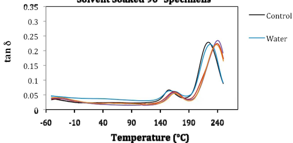
Glass Transition Temperature Measurements for 6-hour Solvent Soaked 90° Specimens
