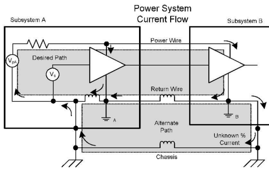
Fig. 2 Uncontrolled power return current
