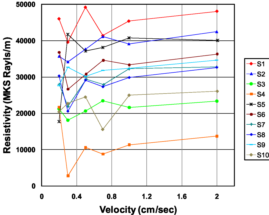
Figure 4. Flow resistivity data for 9.6 kg/m 3 (0.6 pcf) crushed polyimide foam.
