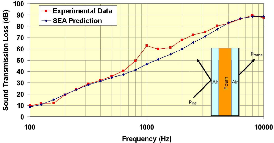
Figure 7. Comparison of the SEA predictions to the experimental data.
