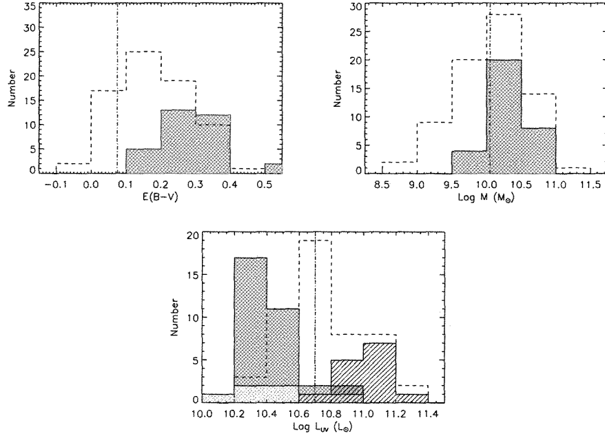
FIG. 8.— Histograms of extinction (left), stellar mass (right) and rest-frame UV luminosity (bottom) for the 32 local LBG analogs. The darker shaded regions highlight the 32 galaxies presented in this paper. A sample of z \sim 3 LBGs (dashed lines) in all three panels are taken from Shapley et al. (2005). The dash-dotted vertical lines show the average extinction (Verma et al. 2007), and stellar mass (Yan et al. 2006) for z \gtrsim 5 galaxies and the typical L_* for z \sim 6 galaxies (Bouwens et al. 2006). (Bottom) The 7 direct detections of LyC flux in LBGs reported in Iwata et al. (2008) are denoted by the lighter shaded histogram, and the lined (angled) histogram shows the z \sim 3 LBG sample of Shapley et al. (2006). The extinction and stellar mass for the COSMOS sources were estimated in the photometric redshift fitting (Mobasher et al. 2007), and the UV luminosity from the GALEX NUV (Zamojski et al. 2007). The histograms show that the galaxies presented in this paper have low levels of extinction, similar stellar masses and rest-frame UV luminosities compared to z \sim 3 LBGs.
