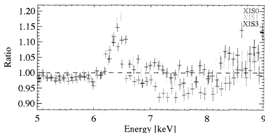
FIG. 4. — Data/model residuals focusing on the iron K bandpass for 2007 when the continuum is modeled as in Fig. 2b.
