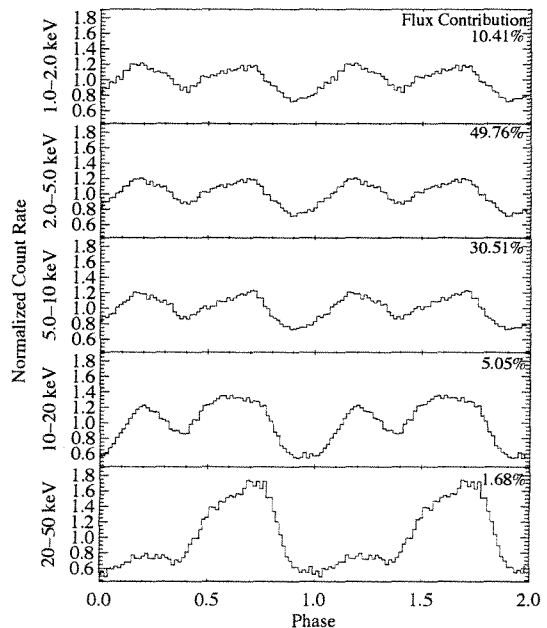
FIG. 7.— Energy resolved pulse profiles for the co-added XIS and PIN data from 2007. Flux contributions are listed for each energy band, representing the percentage of the total flux contributed by that energy range.
