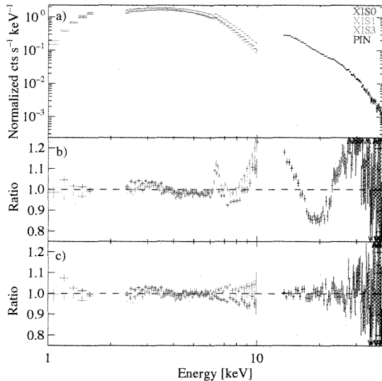
FIG. 2. — Time-averaged spectral fitting for 2007. Panel a) shows the data, three XISs and the PIN. Panel b) the data/model residuals for an absorbed continuum model with FDCut. Panel c) shows the data/model residuals for our best-fit model including the iron lines, 10 keV feature and the CRSF.
