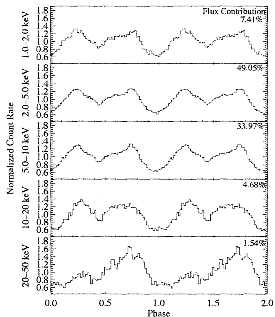
FIG. 6.— Energy resolved pulse profiles for the co-added XIS and PIN data from 2006. Flux contributions are listed for each energy band, representing the percentage of the total flux contributed by that energy range.
