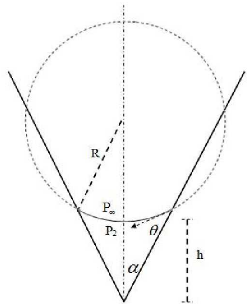
Figure 3: Liquid in a wedge
