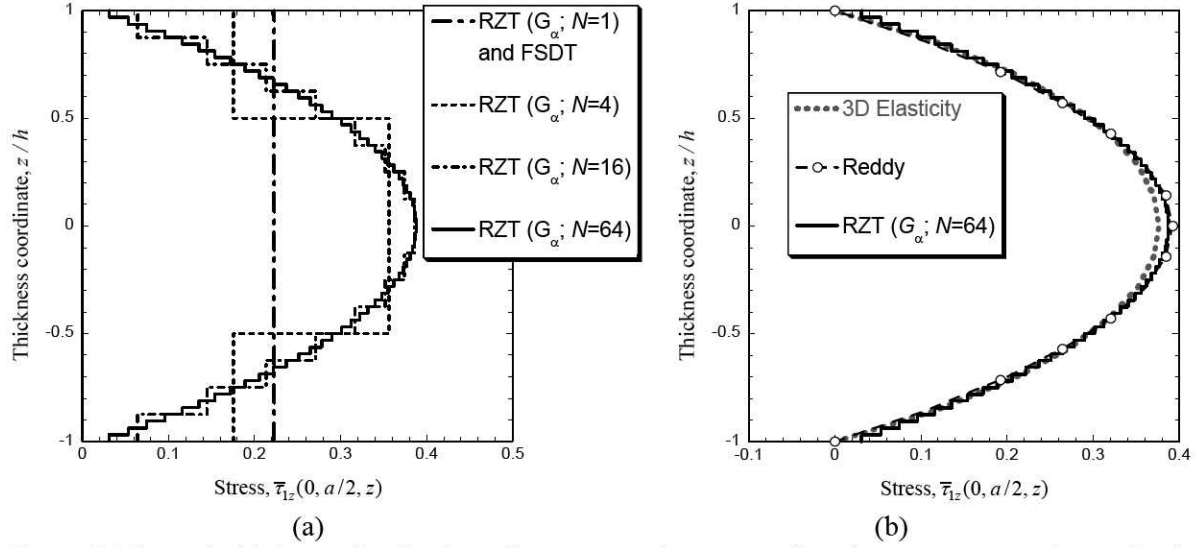
Figure 5. Through-the-thickness distribution of transverse shear stress for a homogeneous orthotropic plate ( a/2h=5 ).
