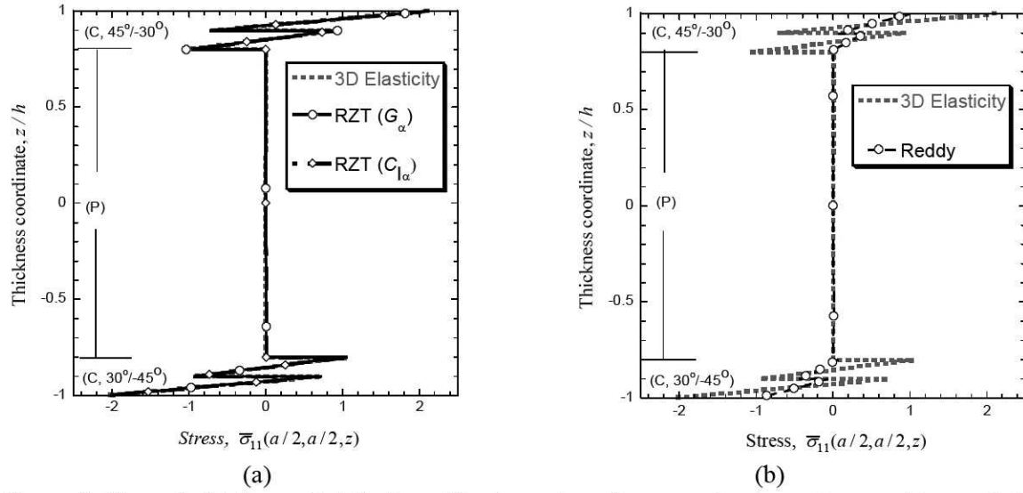
Figure 7. Through-thickness distribution of inplane stress for an angle-ply, antisymmetric, sandwich laminate ( a/2h=5 ).
