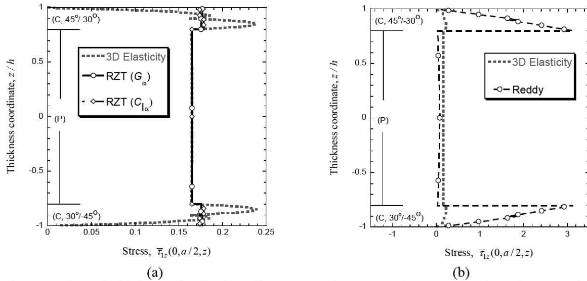
Figure 8. Through-thickness distribution of transverse-shear stress for an angle-ply, antisymmetric, sandwich laminate ( a/2h=5 ).
