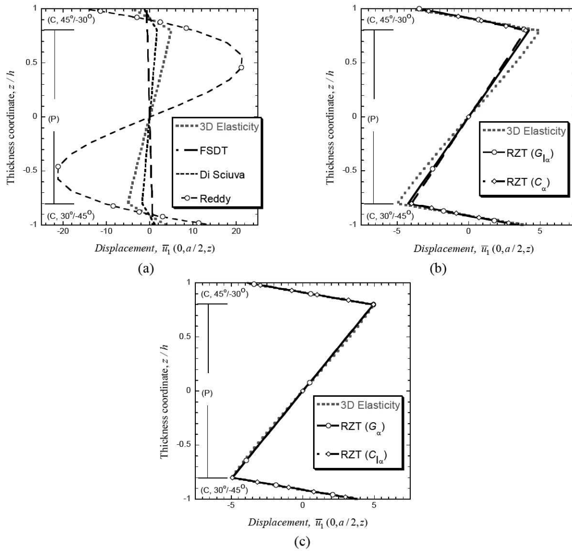
Figure 6. Through-thickness distribution of inplane displacement for an angle-ply, antisymmetric, sandwich laminate ( a/2h=5 ).
