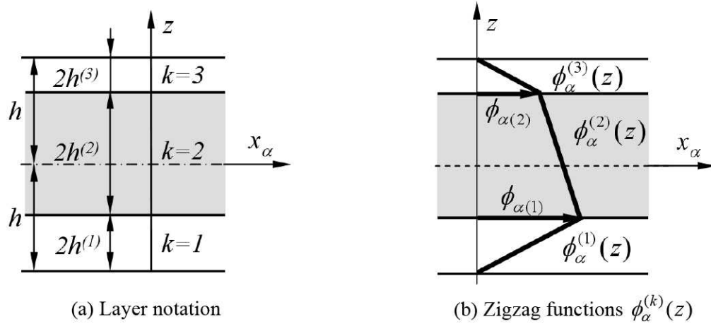
Figure 2. Notation for a three-layered laminate and \phi_\alpha^{(k)}(z) zigzag functions defined in terms of interface displacements \phi_{\alpha(k)} .
