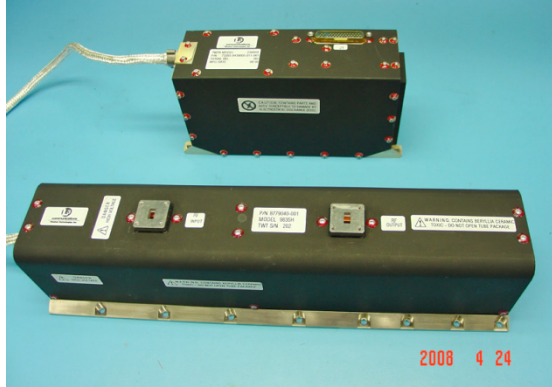
Figure 1.—Photograph of the LRO 40-W K-Band traveling-wave tube in a conduction cooled package attached by an umbilical power cord to an electronic power conditioner located in the background. The TWT input/output waveguide ports are WR-34.
