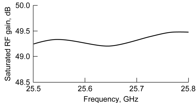
Figure 3.—Measured saturated RF gain as a function of frequency.
