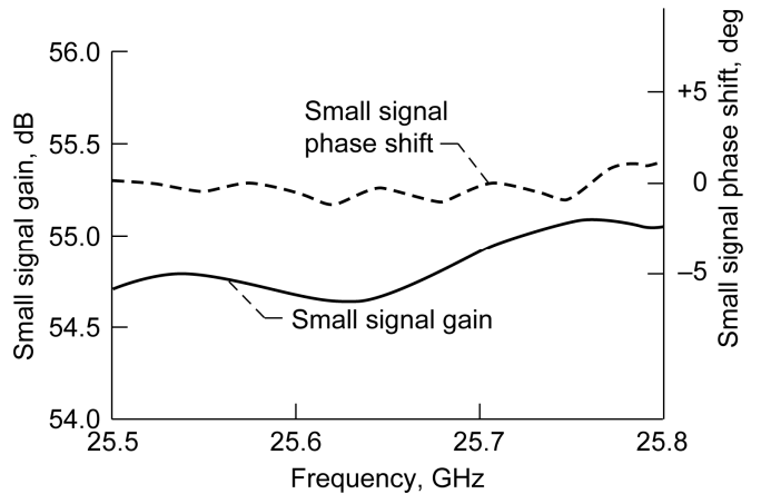
Figure 6.—Measured small signal gain and phase shift as a function of frequency.
