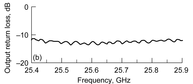
Figure 7.—Measured return loss as a function of frequency. (a) Input port (b) Output port.
