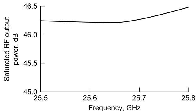
Figure 4.—Measured saturated RF output power as a function of frequency.
