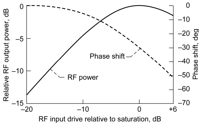
Figure 2.—Measured relative RF output power and phase shift as a function of the RF input drive relative to saturation at the center frequency of 25.65 GHz.
