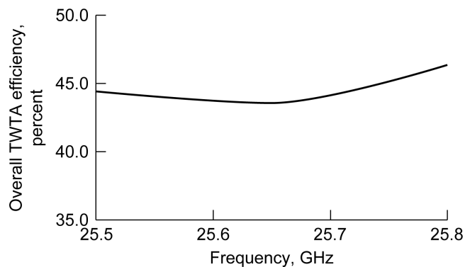
Figure 5.—Measured overall TWTA efficiency as a function of frequency.
