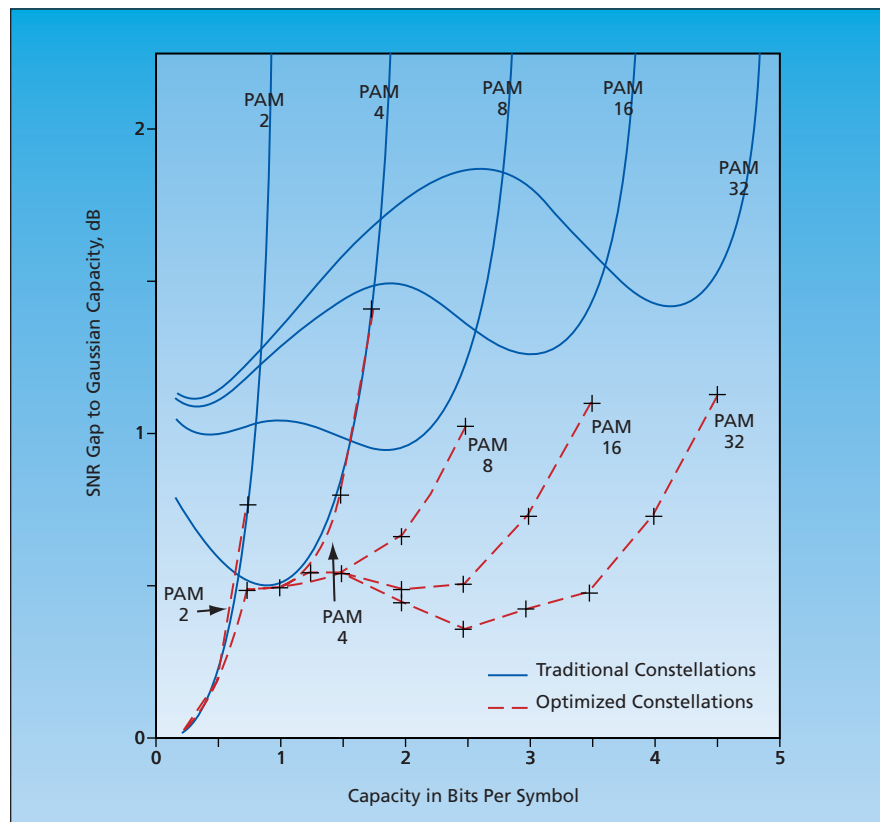
Gaps Between Parallel Decoding Capacity and Gaussian Capacity [quantified as equivalent signal-to-noise-ratio (SNR) gaps] were computed for optimized and traditional PAM 2-, 4-, 8-, 16-, and 32-point constellations.
