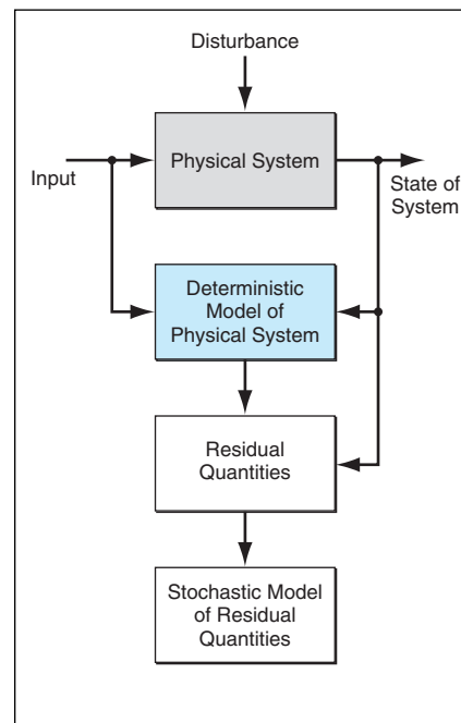
In the Gray-Box Method , the present POD-based method is used to construct a low-order deterministic model that closely approximates the behavior of the physical system.
