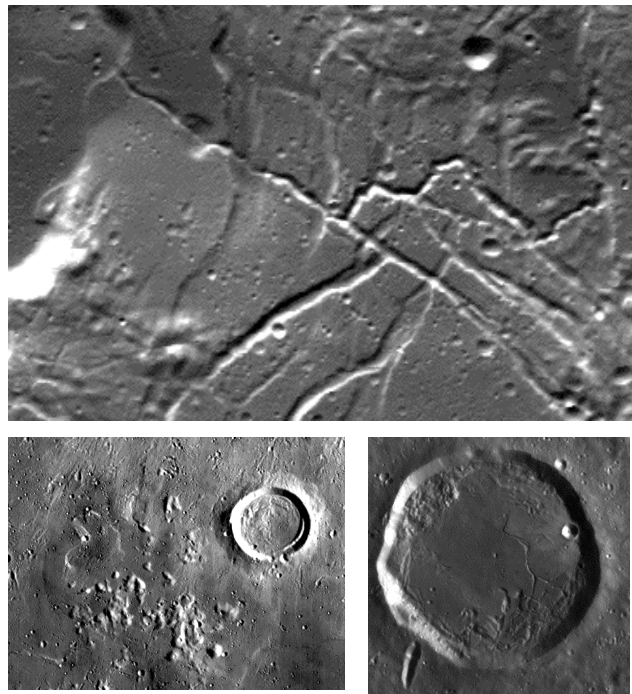
Fig. 1. M3 images from 2.9 \mu\text{m} mosaic: A, top: Sinuous rille entering MO (left) from a fracture in the impact melt (MF); vent region (upper right), parts of graben floors (middle), and MO (left) show mare basalt spectral characteristics; north is to left, image \sim 48 km wide. B, lower left: Shield volcano-like vents in central MO west of Hohmann crater (16 km). C, lower right: Kopff Crater (41 km) showing the exterior with non-volcanic spectral affinities and the volcanically modified interior.
