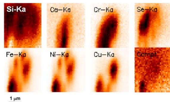
Fig. 3: X-ray fluorescence and Compton map of I1043,1,30.
