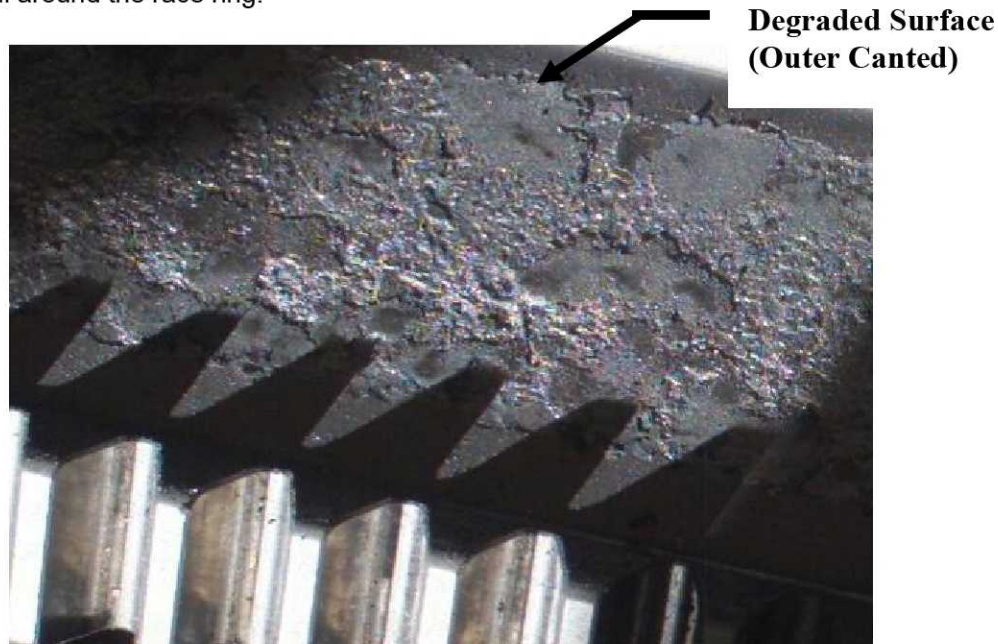
Figure 3: Degradation of the on-orbit SARJ race ring
