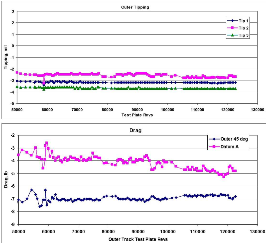
Figure 14: Tipping & drag vs revs
