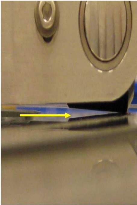
Figure 8: Tipped roller
