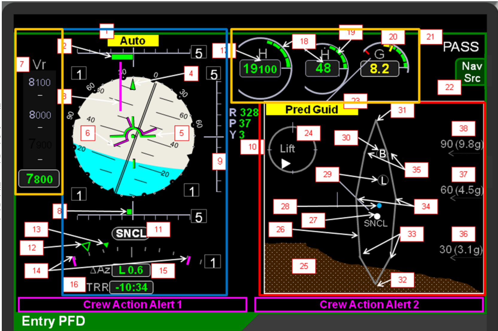
Figure 2 Orion Primary Flight Display.
