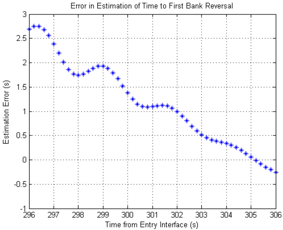
Figure 10 Errors in estimation of time to first bank reversal.
