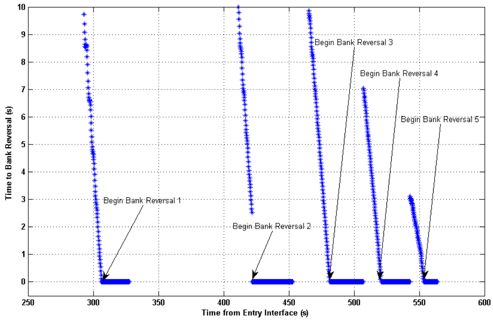
Figure 9 PredGuid Time to Bank Reversal
