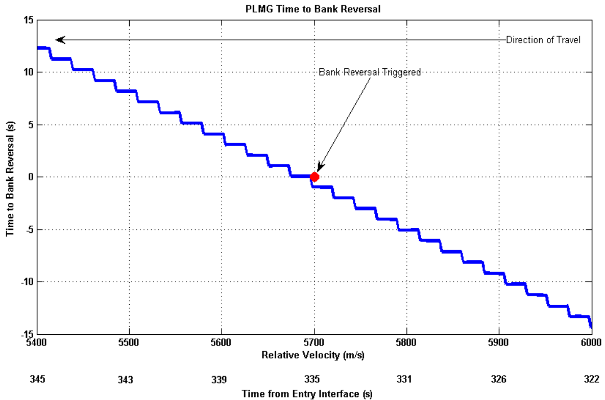
Figure 11 Time to Bank Reversal on PLMG.
