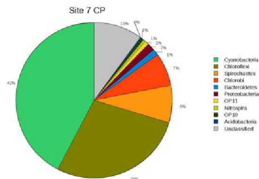
Fig. 1. Microbial diversity in a cyanobacterial mat determined by 16S clone libraries in IDHS Chocolate Pots (Yellowstone National Park, WY, USA). T- 52°C, [Fe 2+ ] – 77 μM, pH – 5.7.
