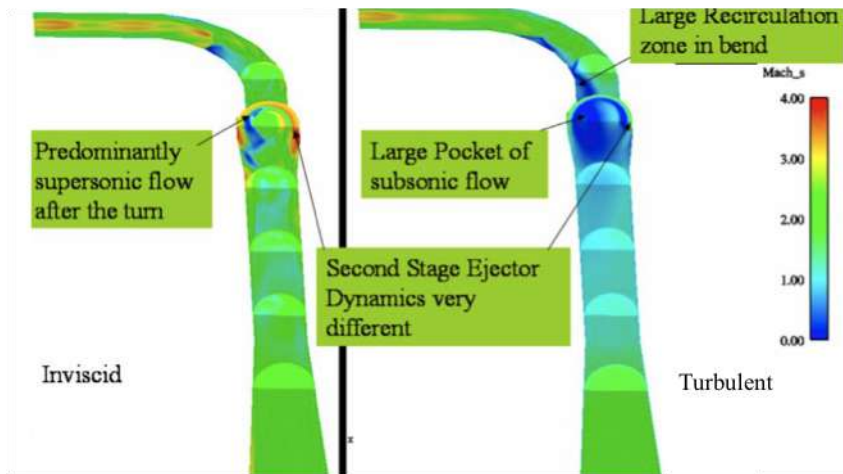
Figure 3. Comparison of Mach No. Distribution for the second set of simulations – Inviscid Real Gas Simulation (Left) and Turbulent Real Gas Simulation (Right).
