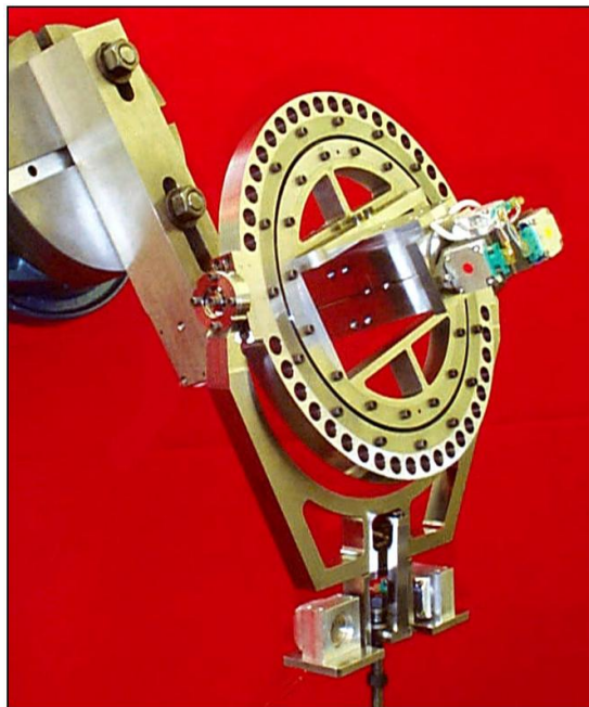
Figure 12. Single Vector System for balance calibration.
