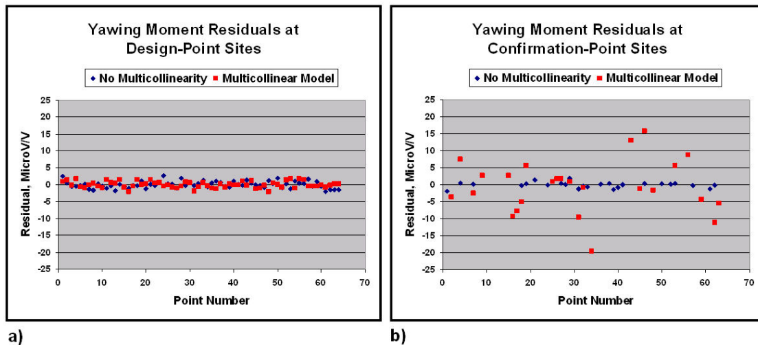
Figure 15. Yawing moment residuals with and without collinear regressors. a) No significant difference in conventional design-point residuals; b) Significant difference at off- design confirmation-point sites.
