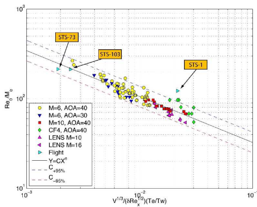
Figure 14. Cavity volume-based correlation for BLT Tool V2
