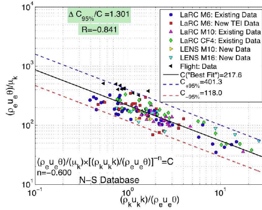
Figure 8. Initial proposed secondary protuberance correlation for BLT Tool V2
