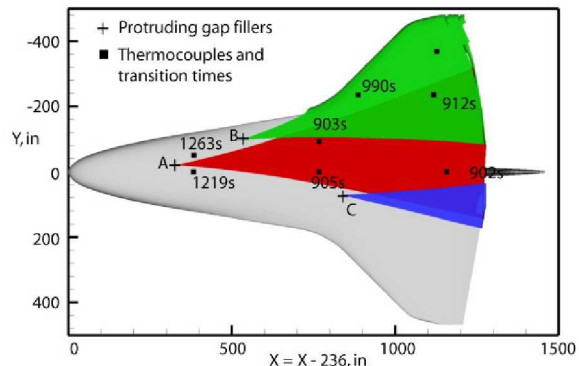
Figure 6. Historical BLT assessment for STS-28
