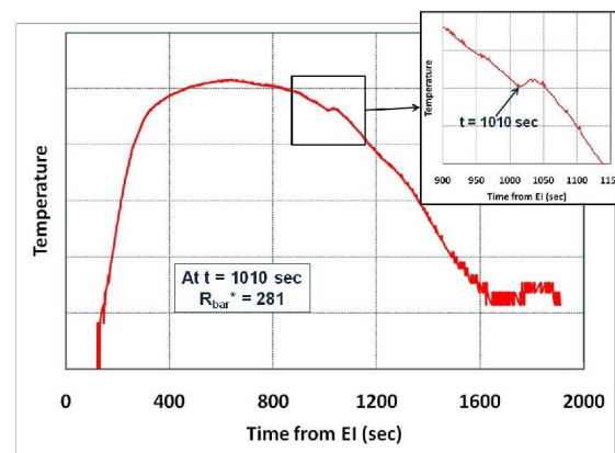
Figure 17. Wing leading edge data on STS-48
