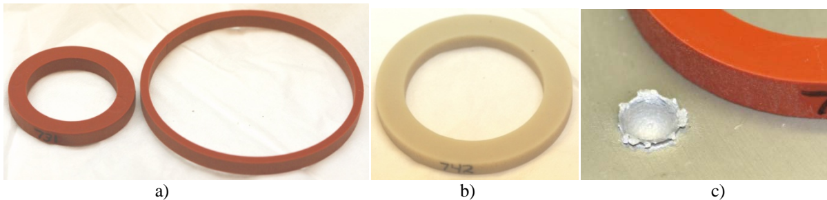
Figure 3. Test articles used in hypervelocity impact tests. a) 5.2 and 2.5 mm wide Parker "ring" seals; b) 9.1 mm wide Esterline "ring" seal; c) anodized aluminum plate cratered by a 1 mm diameter, 1.4 mg, 8 km/s aluminum projectile and a 5.1 mm wide Parker seal.
