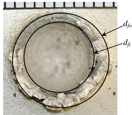
Figure 6. Cratered aluminum plate. Strike 19, the crater in an anodized 6061 T651 aluminum alloy plate resulting from a hit by a 1.58 mm diameter, 5.76 mg, aluminum sphere at 7.9 km/s; the black circles show the inner diameter, d_{fi} , and the outer diameter, d_{fo} ; a mm scale is at the top of the image.
