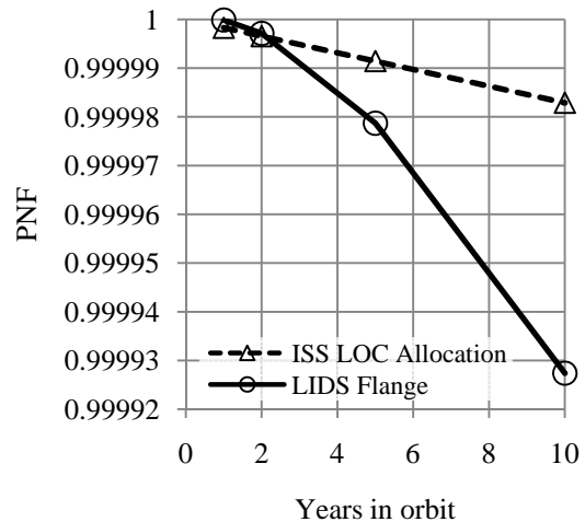
Figure 15. ISS LOC allocation compared to expected risk to the Parker seal. ISS allocation is based on Loss of Crew failure condition, PNF = 0.99999^{4t} ; expected MMOD risks to the Parker flange sealing with the 2.5 mm wide seal for total time in orbit; for example, over 10 years, the ISS flange has received 5 years of ram LEO exposure.
