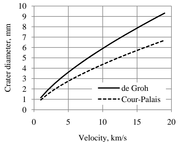
Figure 10. Comparison of the Cour-Palais and de Groh's Eq. (4). Comparison employs 6061 T6 target, and 2017 T4 0.1 cm diameter aluminum projectile.
