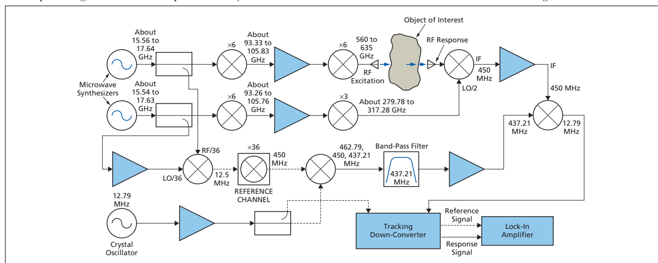
This Vector Measurement System is made from a combination of commercially available and custom components. The complexity of the reference channel is necessitated by a requirement to cancel phase noise that originates in the microwave synthesizers.
