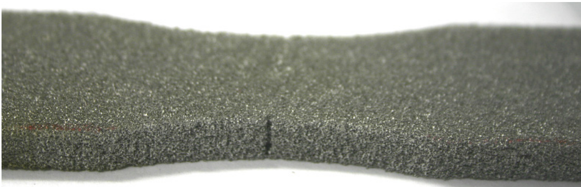
Figure 4.—Repeat rub test on second edge of specimen SS314-80-C. Prior to rub testing a slot was machined in the sample to simulate rubbing over a seam. Remnants of slot visible in center of semi-circular wear pattern. The specimen is 9 mm thick and the rubbed area is approximately 6.3 mm deep.
