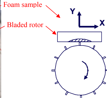
Figure 2.—Illustration of rub test set up. Dashed area indicates area where material is removed.
