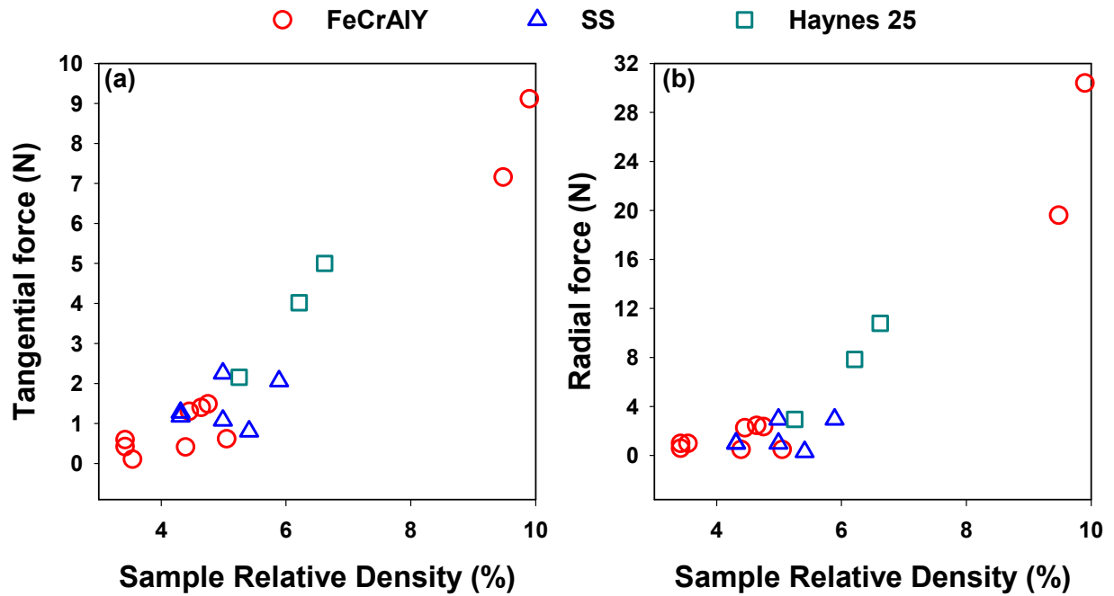
Figure 7.—Rub induced (a) tangential and (b) radial forces as a function of sample relative density.
