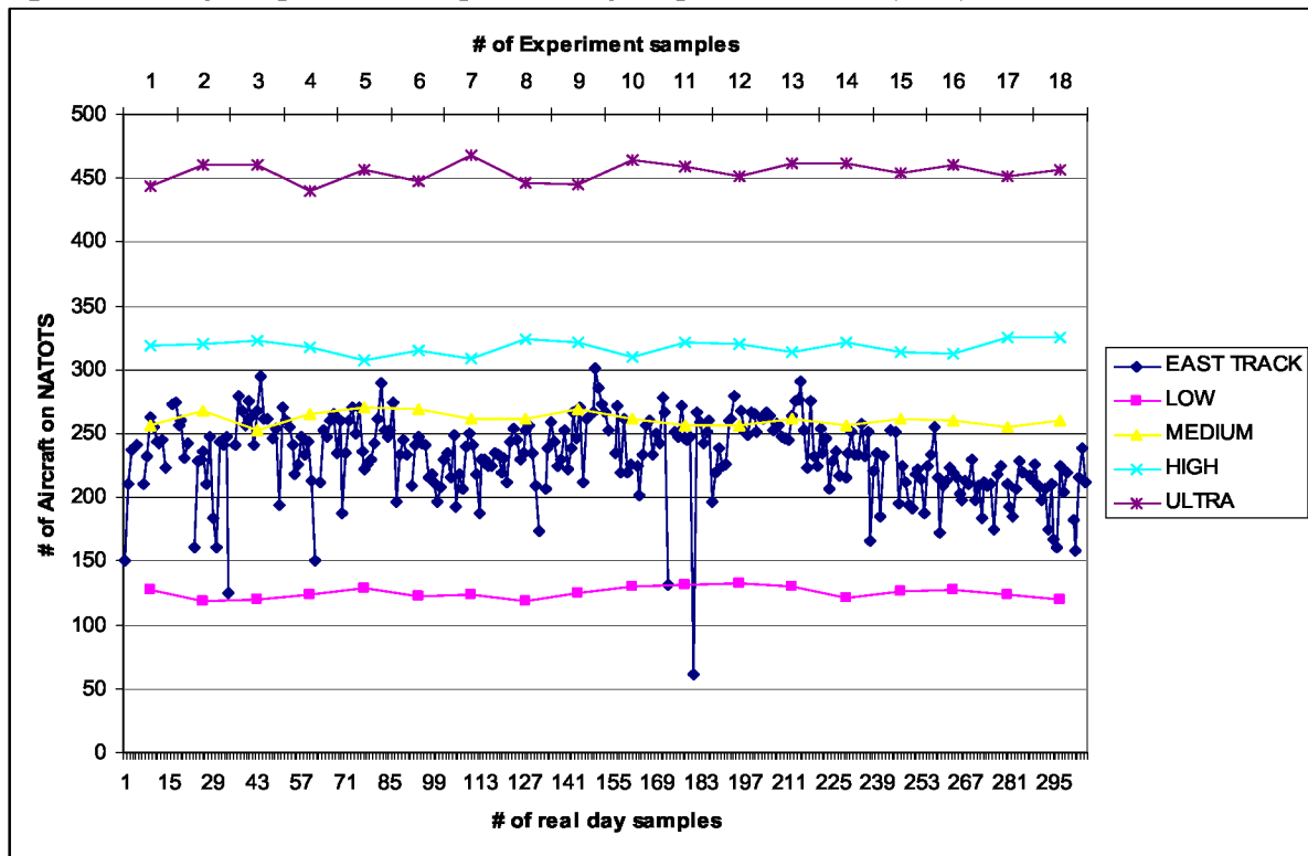
Figure 6: Density comparison for requested entry at optimum altitude (RM0)
