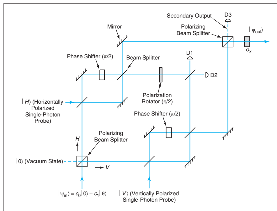
Figure 2. In this Interferometric QND Device , a D1/D2 coincidence accompanied by zero output from D3 would signal the presence of a single photon of arbitrary polarization, which would be preserved.
