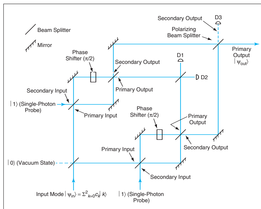
Figure 1. A Single Photon in the Input of this interferometric QND device would be indicated by coincident outputs of photodetectors D1 and D2 and no output of photodetector D3.
