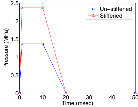
Fig. 7: Pressure histories (blast loads) applied to stiffened and un-stiffened panels.
