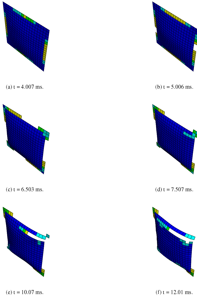
Fig. 8: Failure evolution of un-stiffened composite panel subjected to a blast load.
