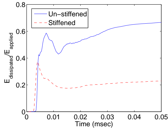
Fig. 13: Energy dissipated due to failure in elements normalized by applied work as a function of time for stiffened and un-stiffened panels.
