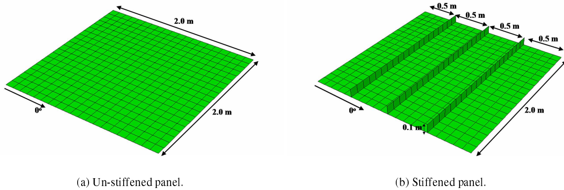
Fig. 5: Meshes used in blast loading of composite panels examples.
