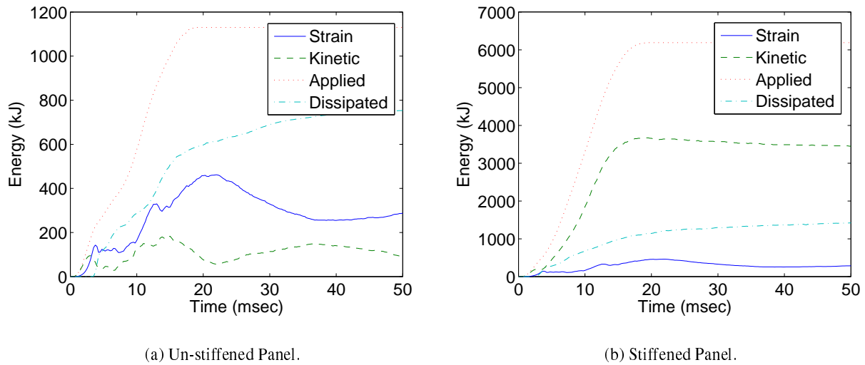
Fig. 12: Energy versus time for stiffened and un-stiffened panels.
