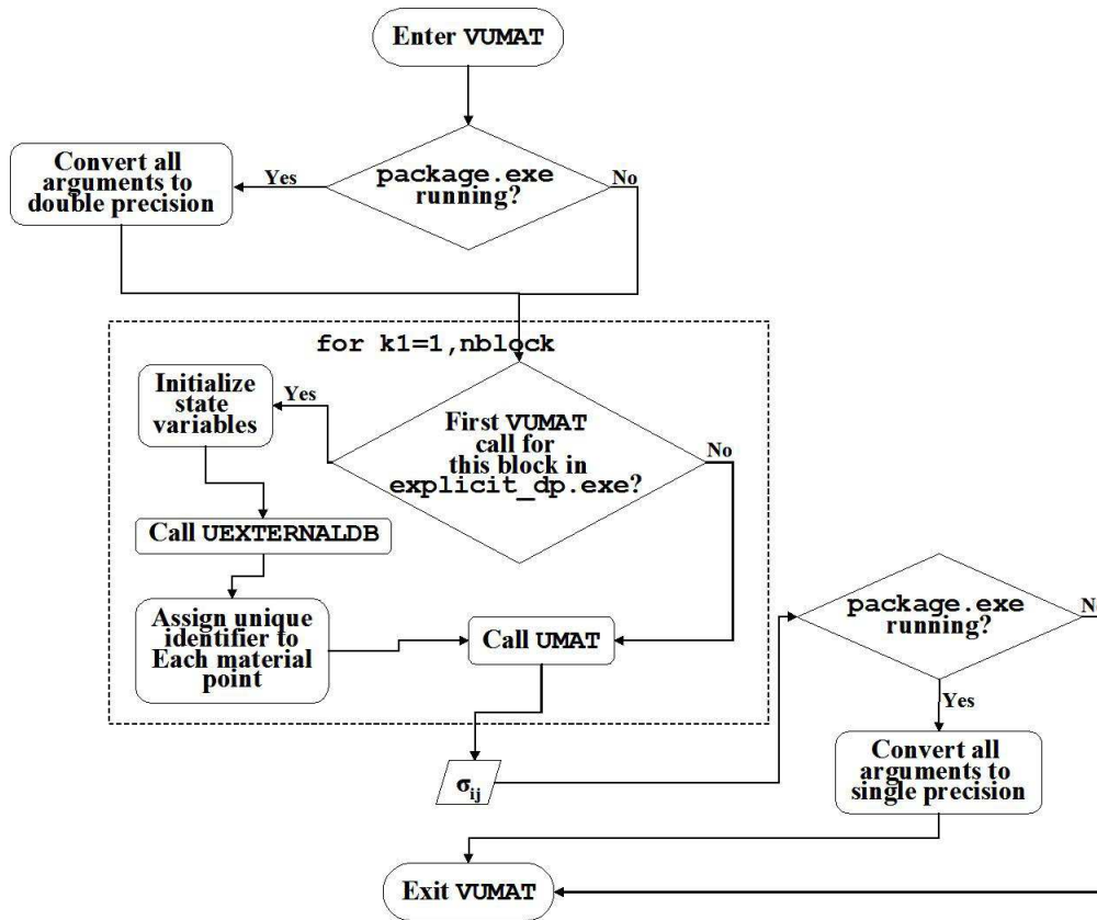
Fig. 4: FEAMAC/Explicit Algorithm.
