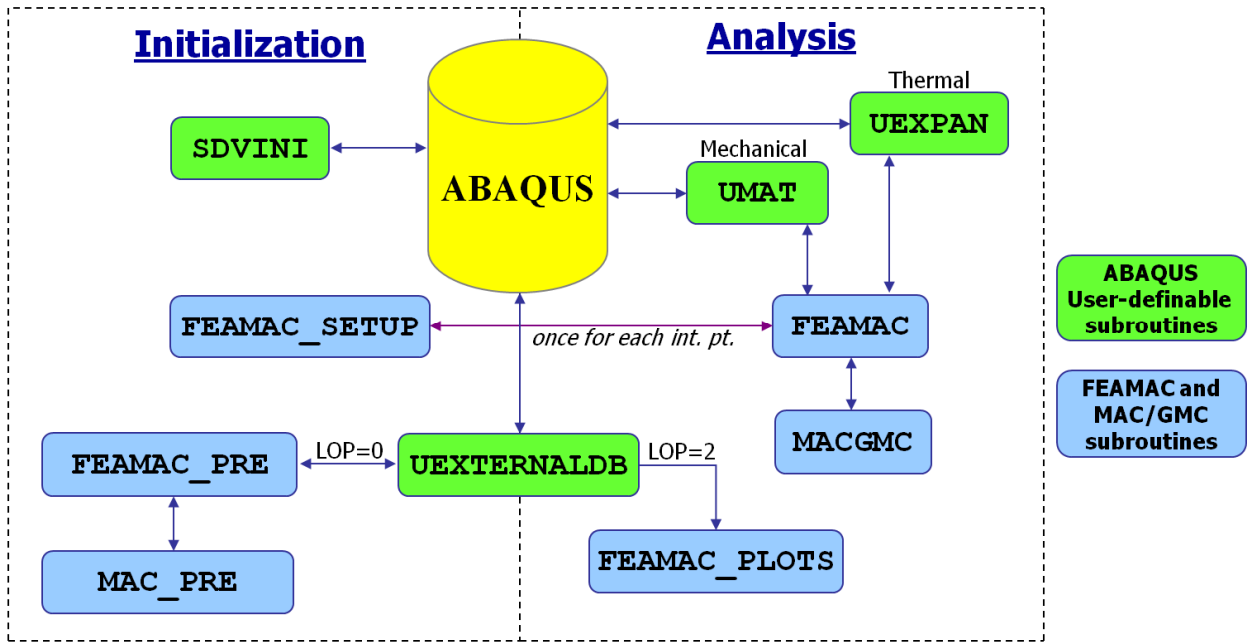
Fig. 2: Hierarchy of FEAMAC software implementation [6].
