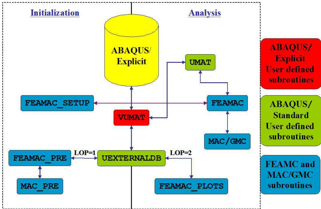
Fig. 3: Hierarchy of FEAMAC/Explicit software implementation.
