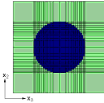
Fig. 1: Demonstrative 26 x 26 GMC RVE.
