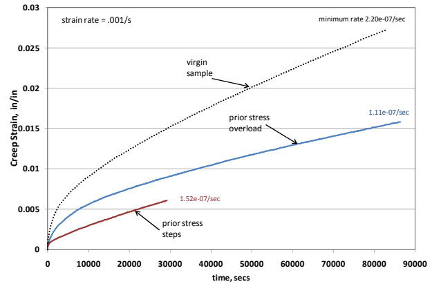
Figure 19. Strain vs. time results from creep tests conducted at 65 ksi and 427 °C to demonstrate history dependence of viscoplastic material behavior.
