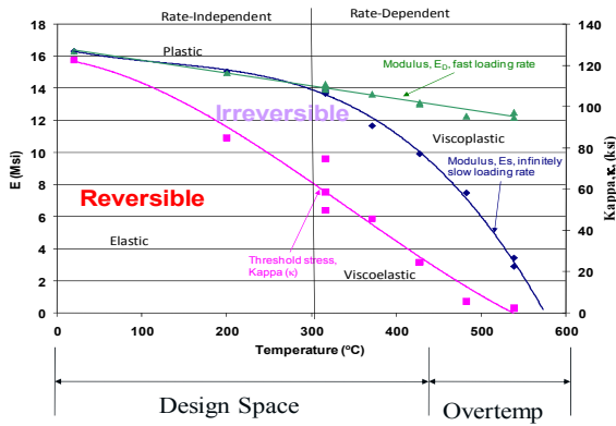
Figure 9: Variation of modulus and threshold stress as a function of temperature for Ti-6-4 material.
