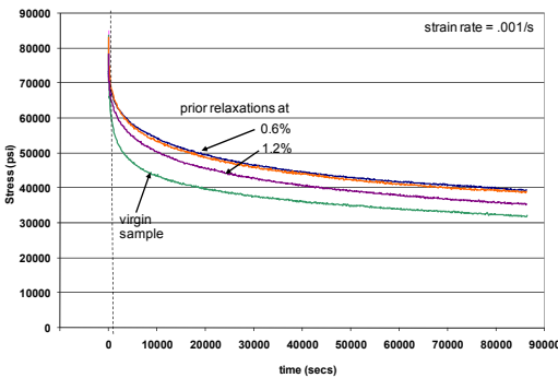
Figure 17: Stress-time results for relaxation at 1.8% strain from relaxation and step relaxation tests conducted at 427 °C to demonstrate history dependence of viscoplastic behavior.
