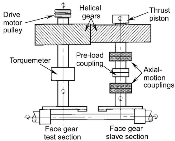
(b) Schematic view.
