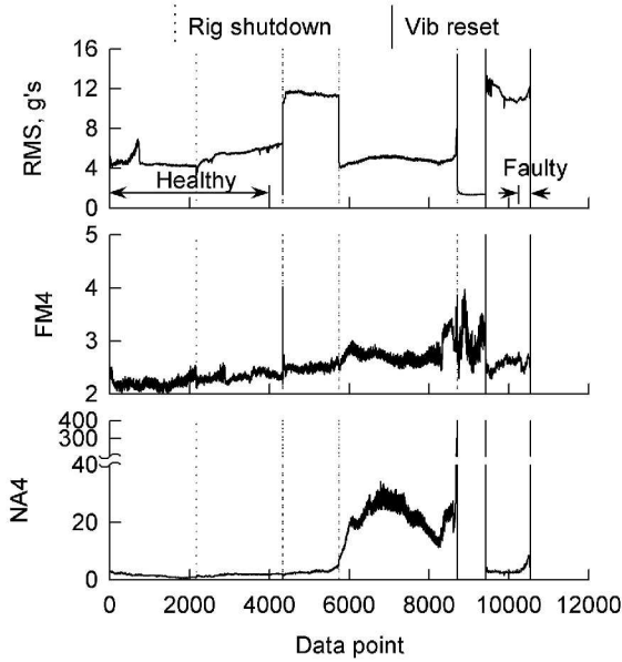
Figure B5.—Set 5 vibration fault detection data.
