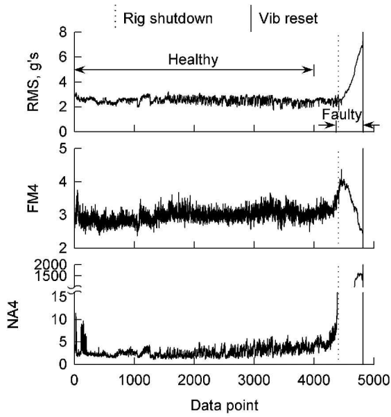
Figure B17.—Set 17 vibration fault detection data.
