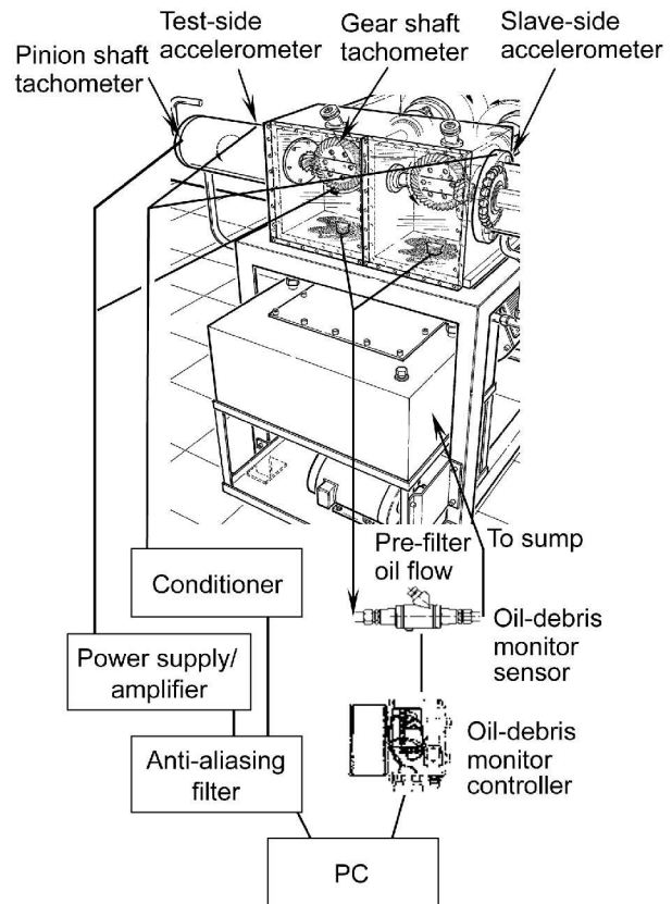
Figure 3.—Gear fault detection instrumentation.
