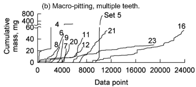
Figure 15.—Oil-debris monitor results.
