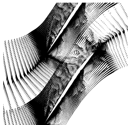
Figure 16(b).—Instantaneous velocity vectors at time step 2, blade tip and near stall condition.
