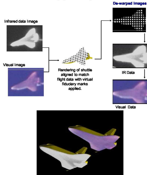
Figure 12. Data de-warping method for texture mapping thermal imagery data to Space Shuttle three-dimensional computer model.
