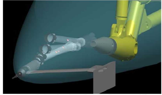
Figure 4. Test setup visualizations used for NASCAR testing, Space Shuttle flow visualization and Ares rocket stage separation testing.
