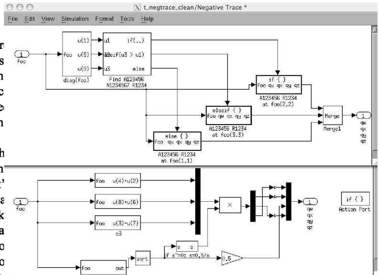
Figure 5. Simulink Model
