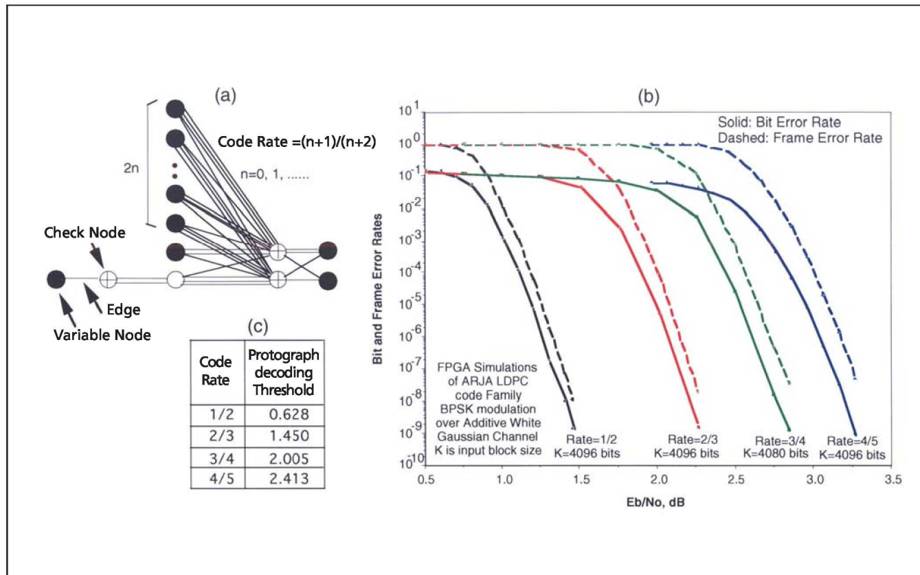
Accumulate-Repeat-Jagged-Accumulate (ARJA) LDPC Code Family is illustrated as follows: (a) protograph, (b) performance of FPGA hardware decoder, and (c) decoding thresholds.
