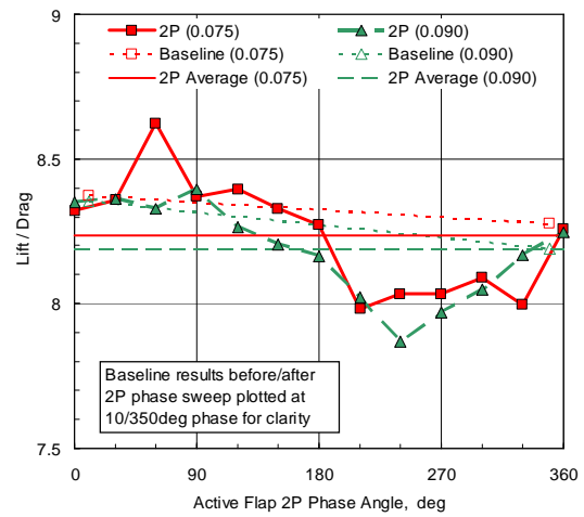
Figure 18b: Rotor performance with active flap inputs of 0 deg and 1.5 deg \sin(2P + \phi) ; \mu = 0.3, \alpha = -9.1^\circ, C_T/\sigma = 0.075, 0.09
