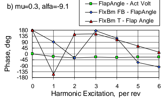
Figure 8: Phase relationships for excitation at rotor speed multiples; active flap vs voltage and flexbeam flap bending and torsion vs active flap
