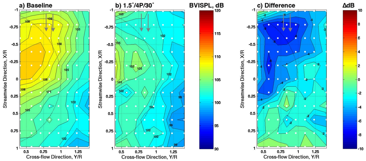
Figure 10a: BVISPL contours for baseline (0 deg) and active flap actuation ( 1.5^\circ/4P/30^\circ ) for Condition 1 ( \mu = 0.150 , \alpha = +4.0^\circ )
