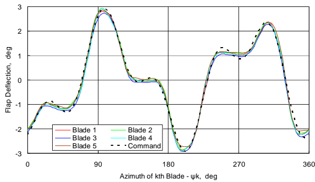
Figure 6b: Active flap deflection versus azimuth at 83 knots, \alpha = 0.89 deg, \delta_f = 1.5 \text{ deg} \sin(2\psi+240) + 1 \text{ deg} \sin(5\psi+330)
