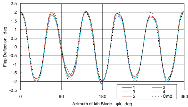
Figure 6c: Active flap deflection versus azimuth at 123 knots, \alpha = -9.4 deg, \delta_f = 2 \text{ deg} \sin(5\psi+90)
