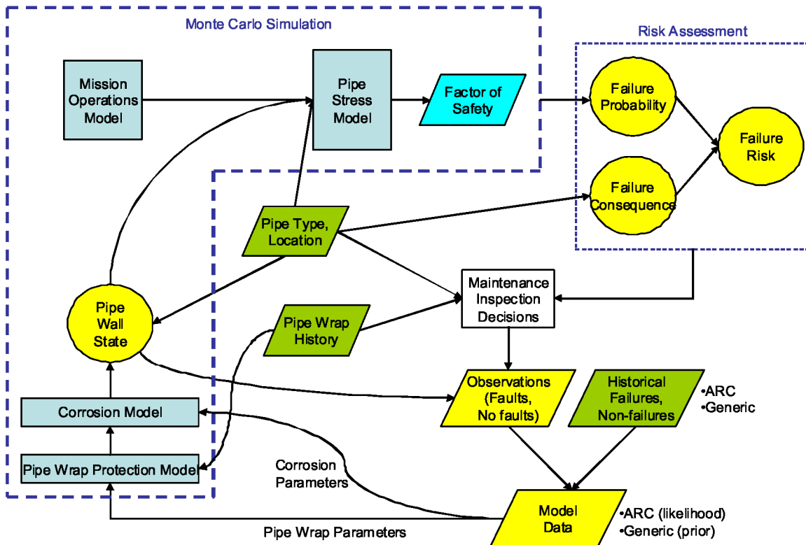
Figure 1: Underground Piping Risk Model.
