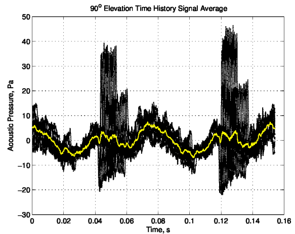
Fig. 29. Uncorrected out of plane time-history signals: averaged (yellow), unaveraged (black).
