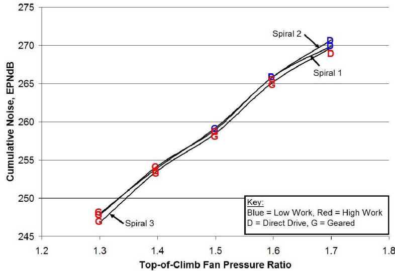
Figure 5. Variation of cumulative noise with fan pressure ratio.
