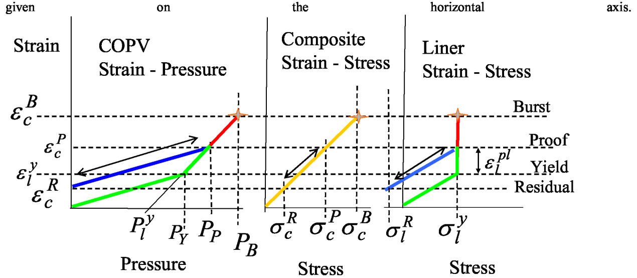
Figure 2. Strain– pressure/stress relationships based on continuity of strain for a COPV, it’s composite and its liner respectively. Operational loads from P=0 to MEOP lie on the blue line for pressures less than P_P
