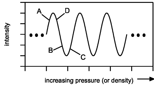
Figure 3. Plot showing the notional response of the interferometer as a function of increasing pressure and/or density (at constant temperature).
