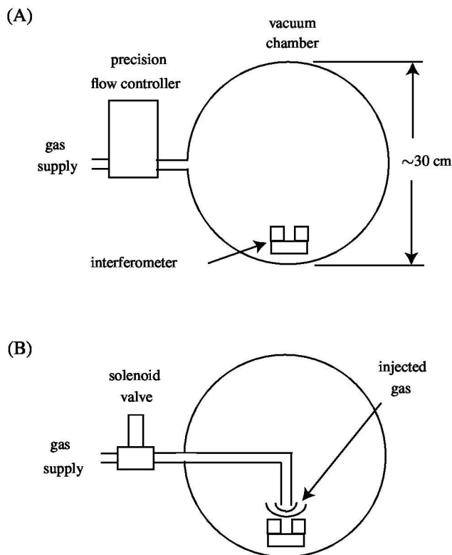
Figure 2. Schematic of the experimental apparatus used for (A) controlled gas injection testing and (B) fast, pulsed gas injection testing.
