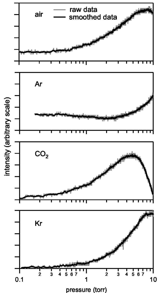
Figure 5. Interferometer measured response to moving interference fringes as a function of pressure (at low pressure levels displayed on a semilog scale) for air, argon, carbon dioxide, and krypton. The intensity scale spans the same range for all plots.
