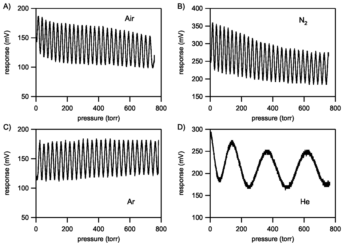
Figure 4. Interferometer measured response to moving interference fringes as a function of pressure (from 0-760 torr) for A) air, B) nitrogen, C) argon, and D) helium.
