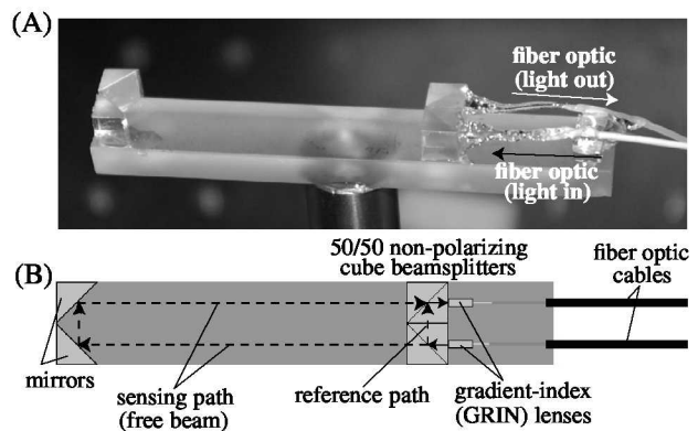
Figure 1. (A) Photograph and (B) schematic of a fiber-coupled gas detection sensor.
