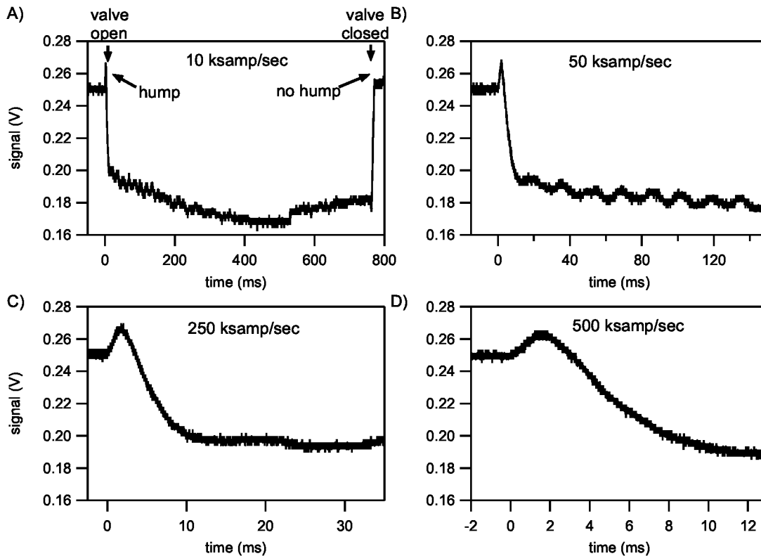
Figure 7. Interferometer response to a short, fast gas pulse injected at the sensor head acquired at A) 10 ksamp/sec, B) 50 ksamp/sec, C) 250 ksamp/sec and D)500 ksamp/sec.
