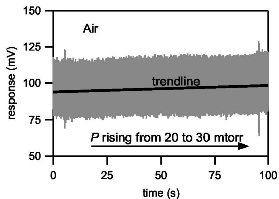
Figure 6. Interferometer response as the vacuum chamber pressure rose from 20 to 30 mtorr due to a slow leak in the vacuum system.
