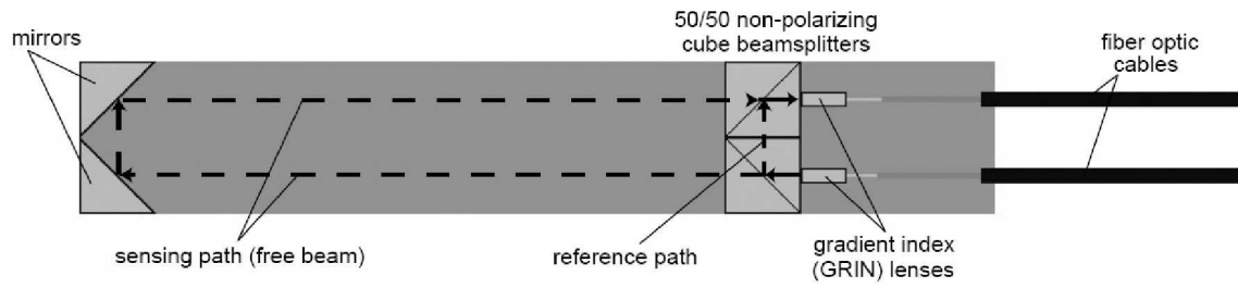
Figure 1. Photograph (top) and schematic (bottom) of a fiber-coupled gas detection sensor.
