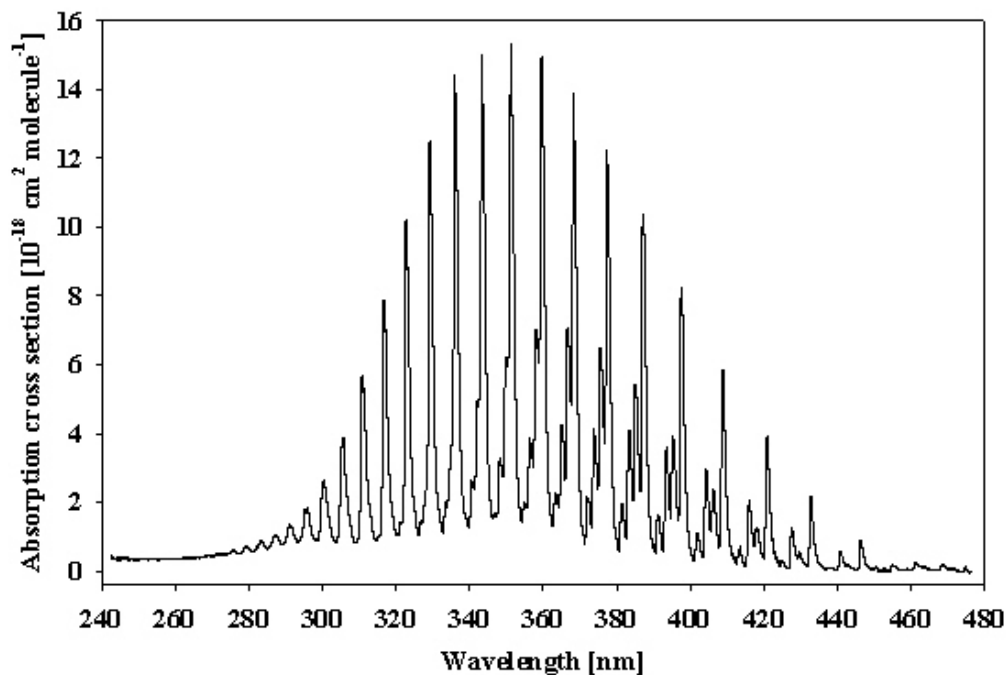
Figure 4-3. Absorption Spectrum of OCIO at 204 K (after Wahner et al. [830])
