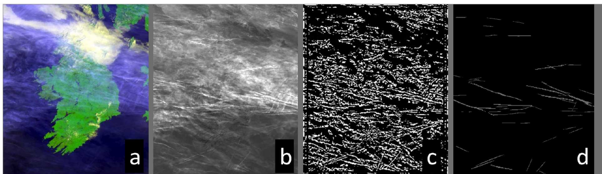
Figure 2: AATSR image for 17/03/2009 at 11:18UTC. a) True colour image, b) 11-12 \mu\text{m} temperature difference image, c) extracted linear features and d) identified contrails ( \sim 2\% coverage).
