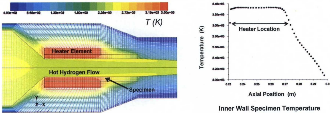
Figure 11. Internal temperature distributions and inner wall surface temperature of specimen.
