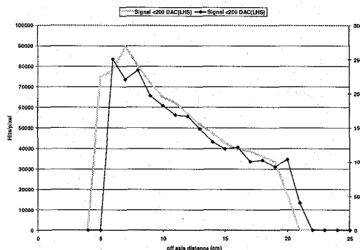
Figure 7: Radial distribution of secondary particles measured by the ZDD. Two distributions are shown for hits: signals <200 ADC channels (left hand scale) and signals >200 ADC channels (right hand scale).
