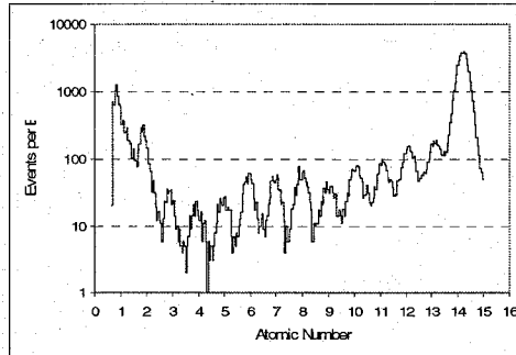
Figure 4: Charge Calibration measurement using a silicon beam. Some fragmentation occurred because of the residual mass on the beam line. Surviving fragments are clearly resolved.
