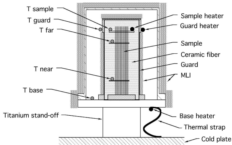
FIGURE 1. The test apparatus in which both the electrical resistivity and thermal conductivity measurements were performed.
