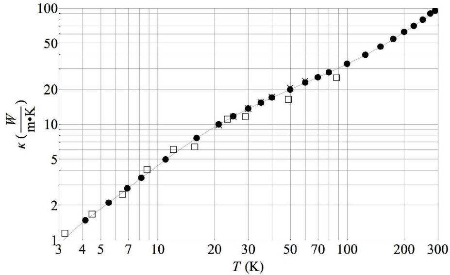
FIGURE 3. Thermal conductivity of phosphor bronze. Solid circles are from this work, using CDA 510 material taken from a JWST cable sample. \times 's are also from this work, but without using the guard can and insulation. Open squares are from Zavaritskii & Zeldovich, 1956.
