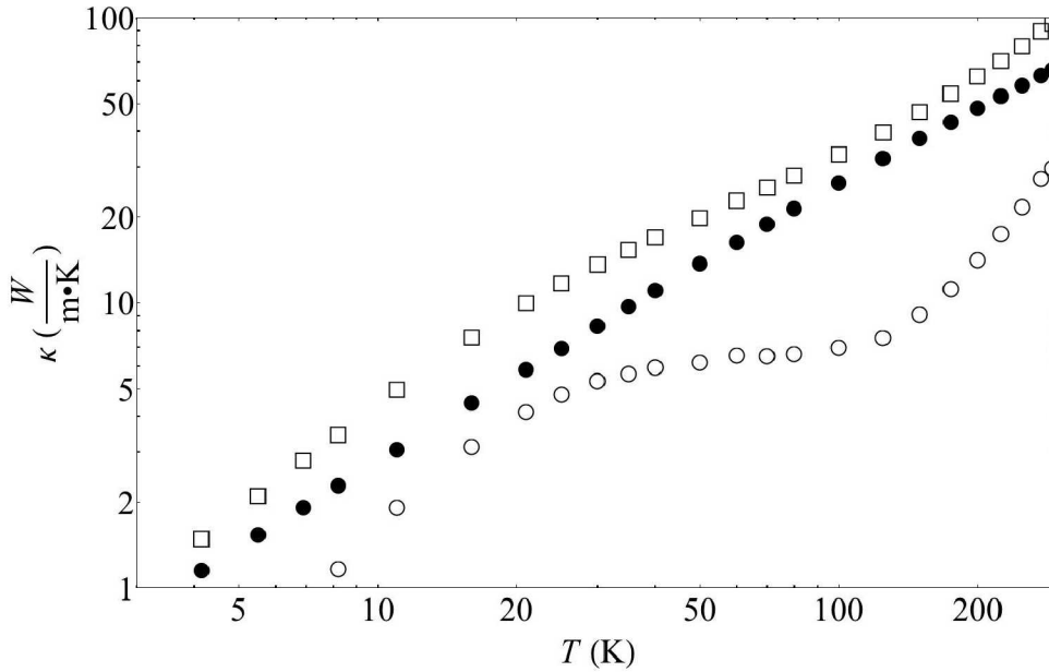
FIGURE 4. The measured total thermal conductivity, \kappa , of CDA 510 phosphor bronze is shown in open squares. Filled circles are the electronic contribution, \kappa_E , as predicted by the Wiedemann-Franz law. The open circles are the phonon contribution, calculated by subtracting \kappa_E from \kappa .
