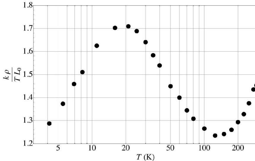
FIGURE 5. The Lorenz ratio L/L_0 , for phosphor bronze CDA 510, Here L is a Lorenz number calculated with the Wiedemann-Franz law using the total thermal conductivity, and L_0 is the fundamental Lorenz constant computed from the elastic-scattering-only electronic thermal conductivity.
