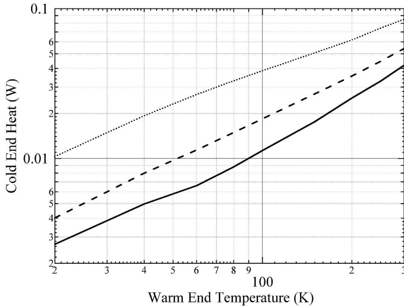
FIGURE 6. The minimum possible heat load at the cold end of an 50 cm long wire conducting 1 amp of current with cold end held at 4 Kelvin. The wire diameter has been optimized at each warm end temperature to minimize the cold end load. Radiation is ignored. The solid line is for 26% drawn copper[10], the large-dash line is for phosphor bronze CDA-510 (this work), and the dotted line is for Hastelloy C-276 TM [5].
