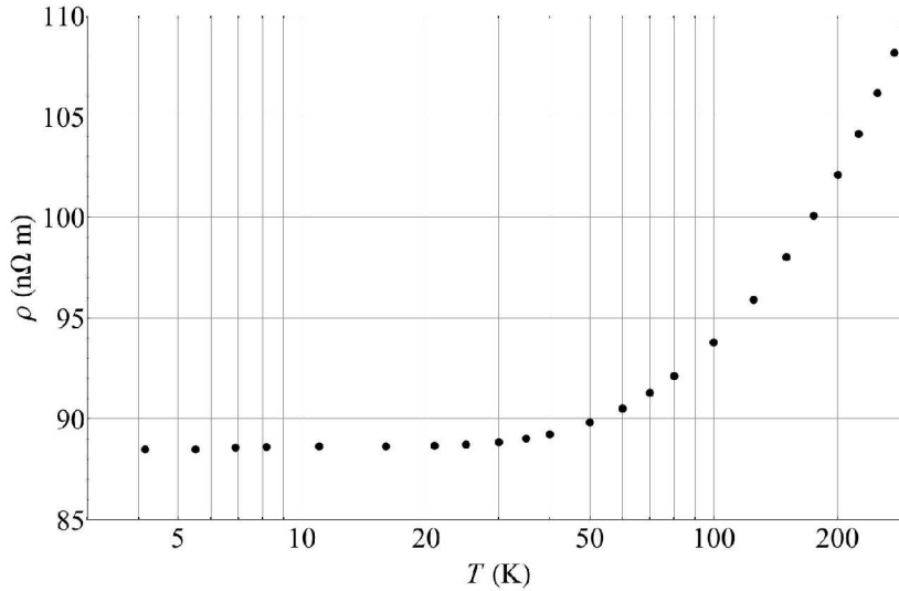
FIGURE 2. The measured electrical resistivity vs. temperature for a phosphor bronze CDA 510 wire from a sample of JWST instrument cabling.
