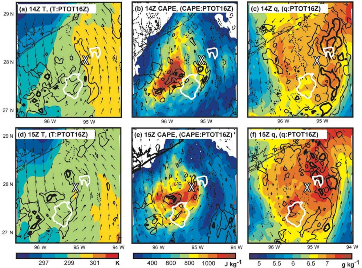
Figure 13. The relationship between PTOT16Z and antecedent (a,d) T sfc , (b,e) MUCAPE and (c,f) mid-level moisture in a Lagrangian, storm centered coordinate system. Ensemble-mean T sfc , MUCAPE, and mid-level mixing ratio (average from 3-6 km) are respectively color filled at intervals of 1 K, 200 \text{J kg}^{-1} , 0.5 \text{g kg}^{-1} at (a-c) 1400 and (d-f) 1500 UTC 12 September. Correlation between the variable in each panel and PTOT16Z is contoured as in Fig. 12. Surface wind vectors are shown in (a-b) and (d-e), and 3-6-km average wind vectors are shown in (c) and (f). The PTOT16Z region is contoured in white, and the bold 'X' represents the position of the mean circulation center at 1600 UTC for reference.
