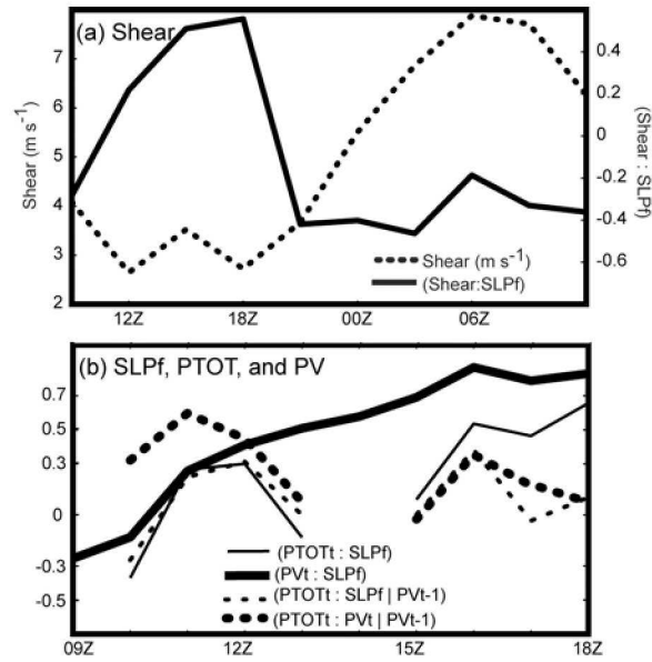
Figure 5. The relationship between storm intensity and (a) wind shear from 0900 UTC 12 September to 1200 UTC 13 September and (b) PV and precipitation from 0900 to 1800 UTC 12 September. In panel (a), wind shear (dotted) and the correlation between wind shear SLPf (solid) are shown. Wind shear is computed as the difference between the mean 200 and 850-hPa wind vectors averaged within 300 km of the circulation center. Until 1800 UTC, shear is calculated from the EnKF analysis, and after that time it is calculated from the ensemble forecast. Panel (b) shows the correlation between 2-km PV within the 2-PVU isopleth and SLPf (thick black), the correlation between SLPf and PTOT (thin black), the correlation between PTOT and SLPf when controlling for 2-km PV at the previous hour (thin dotted), and the correlation between PTOT and 2-km PV when controlling for 2-km PV at the previous hour (thick dotted). All variables are computed in a Lagrangian coordinate system following the storm center.
