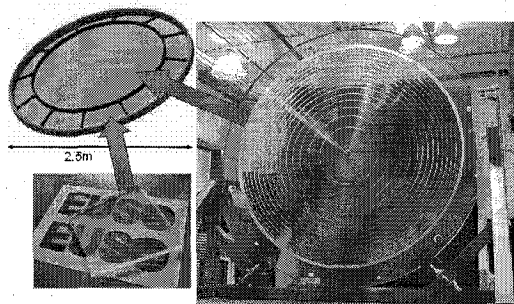
Fig. 2 Fresnel lenses of the JEM-EUSO consisting of a central lens and peripheral petal segments
