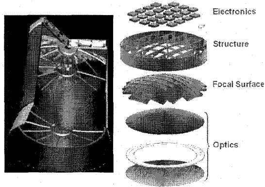
Fig. 1 Configuration of the JEM-EUSO telescope
