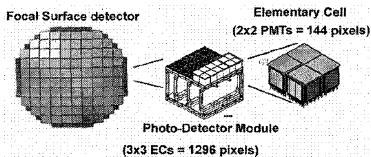
Fig. 3 Focal surface detector
