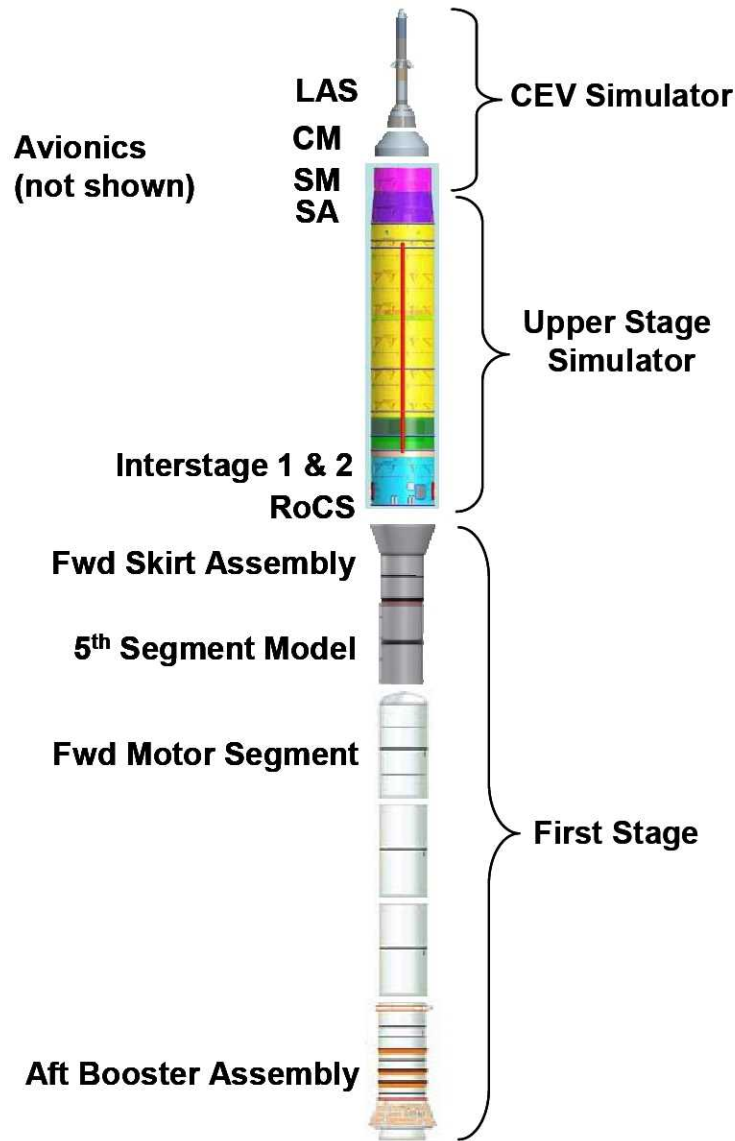
Figure 1. The Ares I-X Vehicle.
